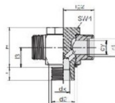
TH - BSP
