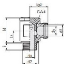
WH - BSP
